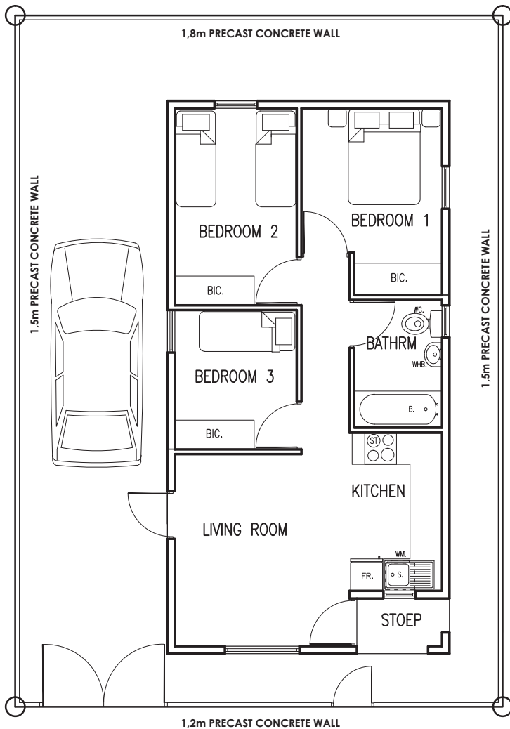
FLOOR PLAN
